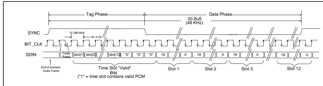
Figure 5-22. AC-link Protocol
