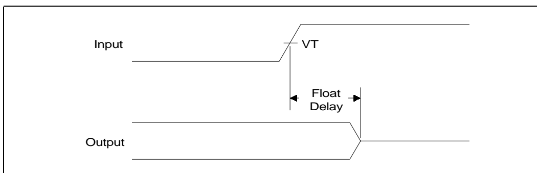
Figure 16-4. Float Delay
