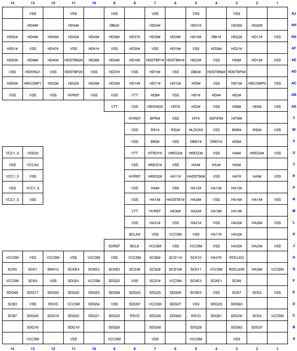
Figure 7. Intel® 82845 MCH Ballout Diagram (Top View—Right Side)
